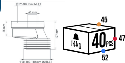
TPTK-EX40 PRODUCT CODE 40 MM EKSANTRİK KADA 40 MM ECCENTRIC PAN CONNECTOR
